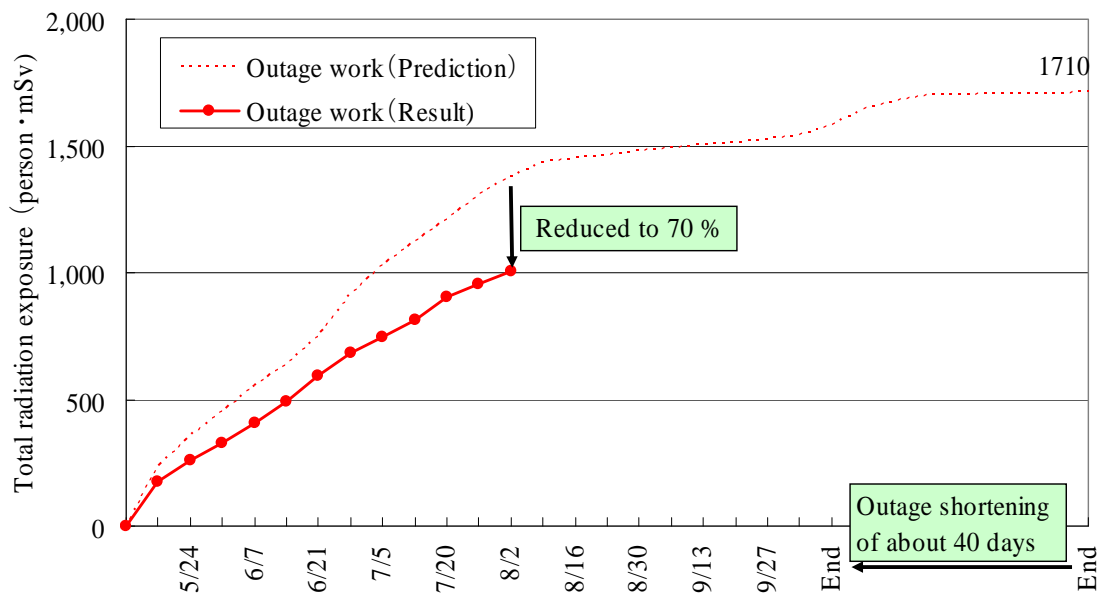
Figure 6 Trend of total radiation exposure during the 28 th outage (Outage works)
