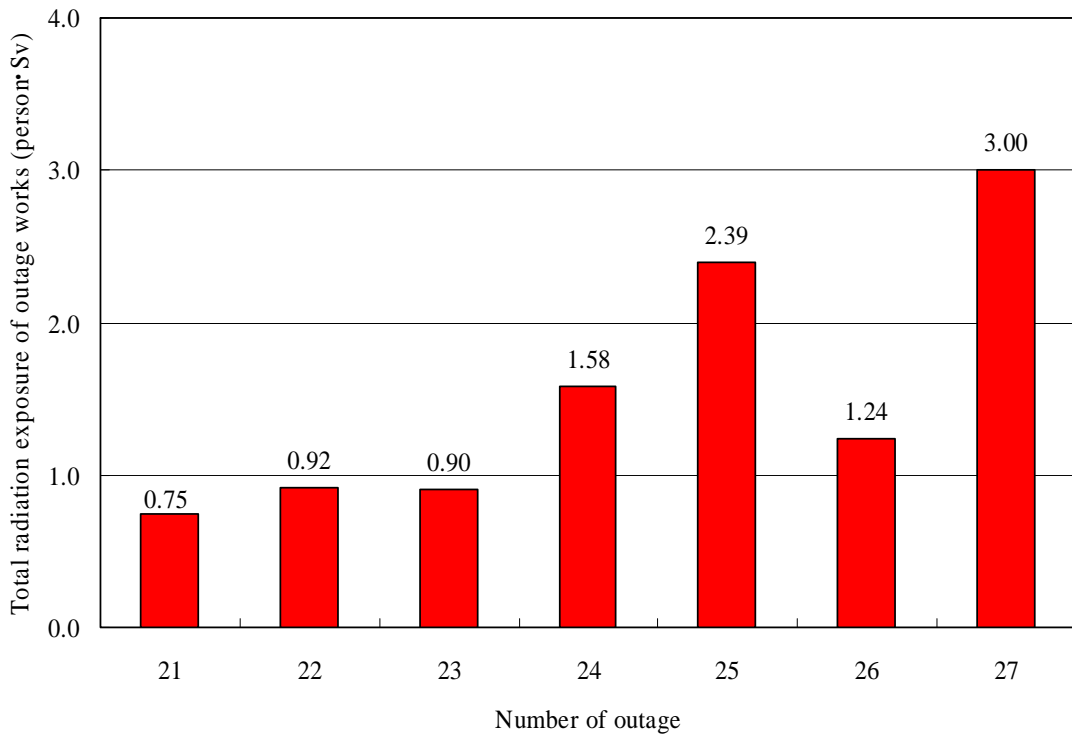
Figure 1 Radiation exposure at Shimane Nuclear Power Station Unit 1 after hydrogen injection
