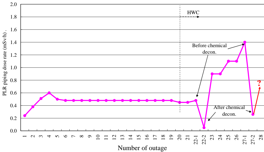
Figure 2 PLR dose rate trend at Unit 1
